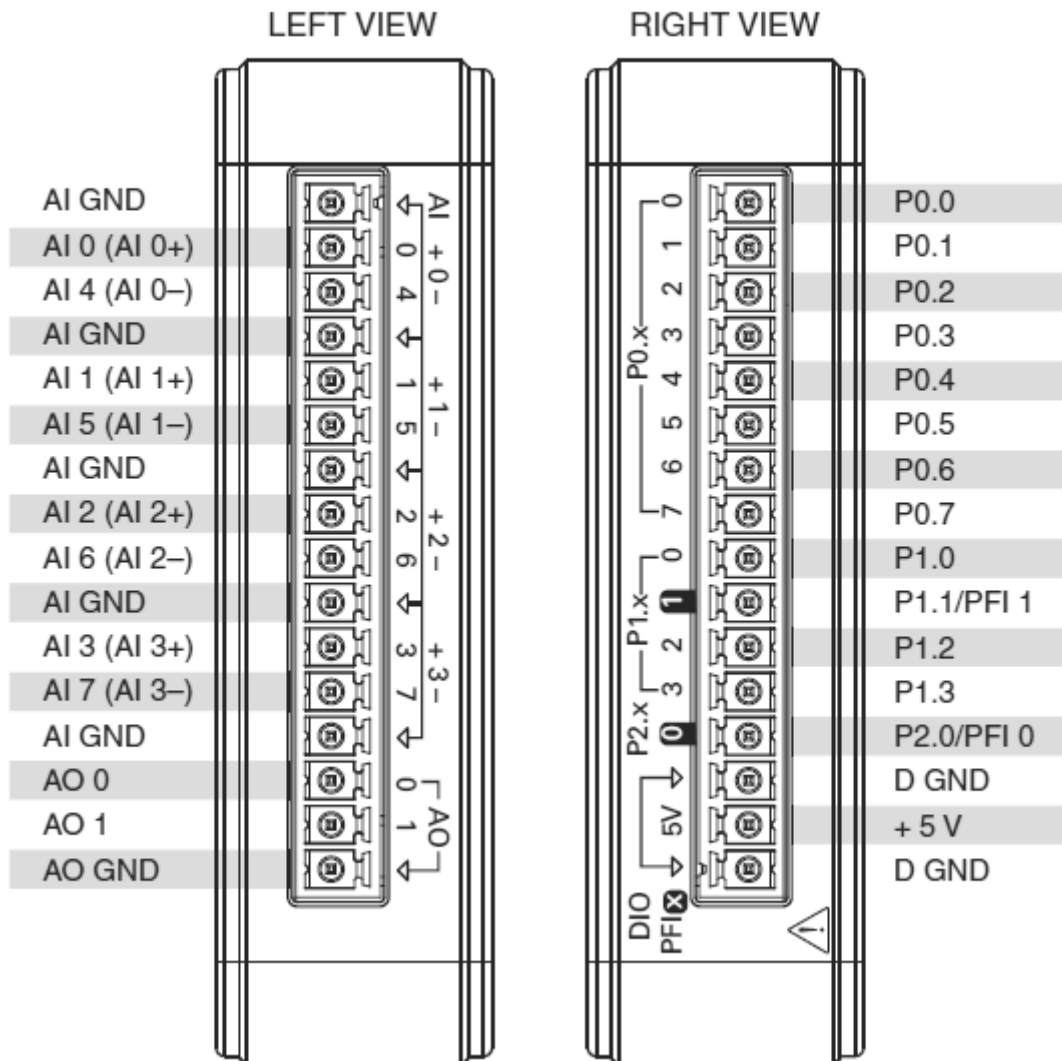
Figure 4. NI USB-6001/6002/6003 Pinout
